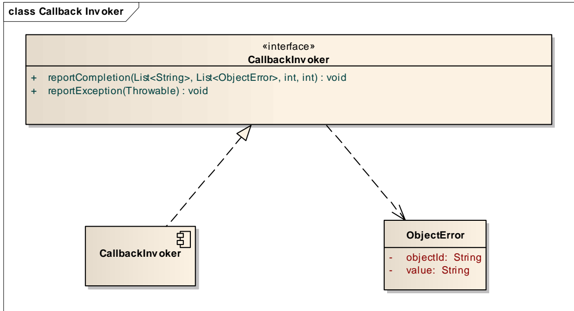
Figure 11 Callback Invoker class
