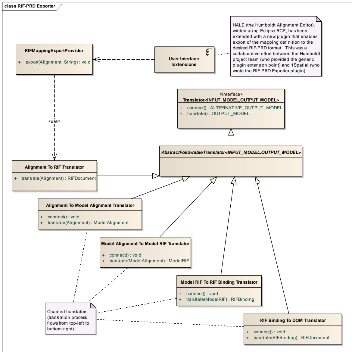
Figure 15 RIF-PRD Exporter class diagram
