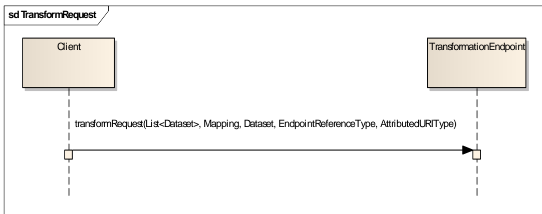
Figure 17 Transform request sequence diagram
