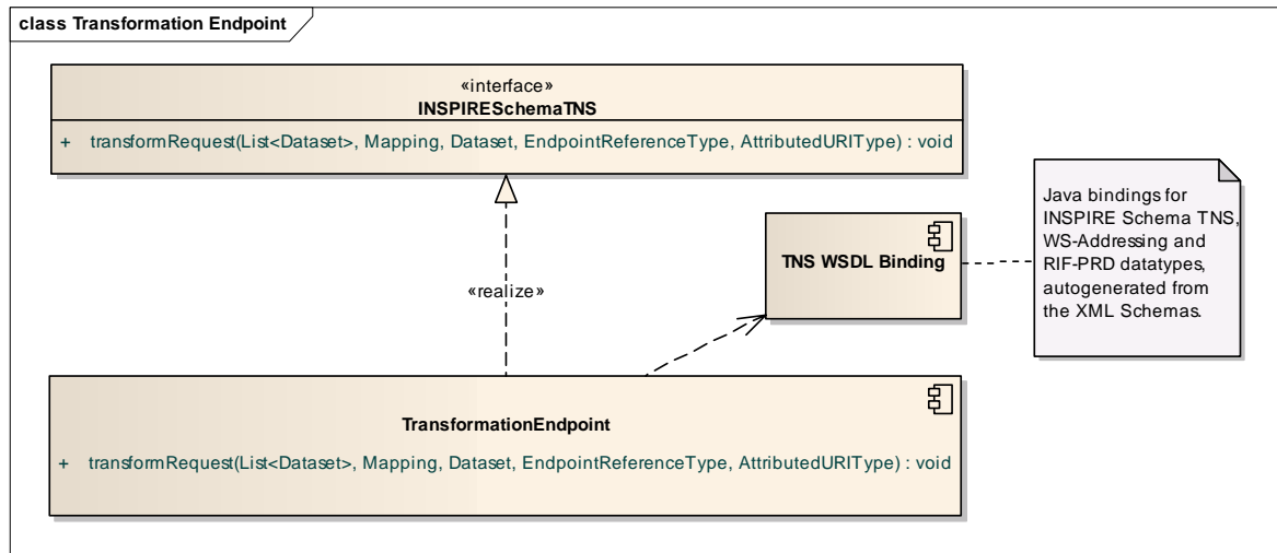
Figure 10 Transformation Endpoint class diagram
