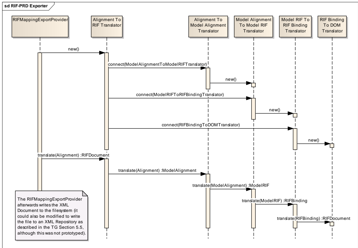
Figure 16 Sequence diagram for RIF-PRD Exporter
