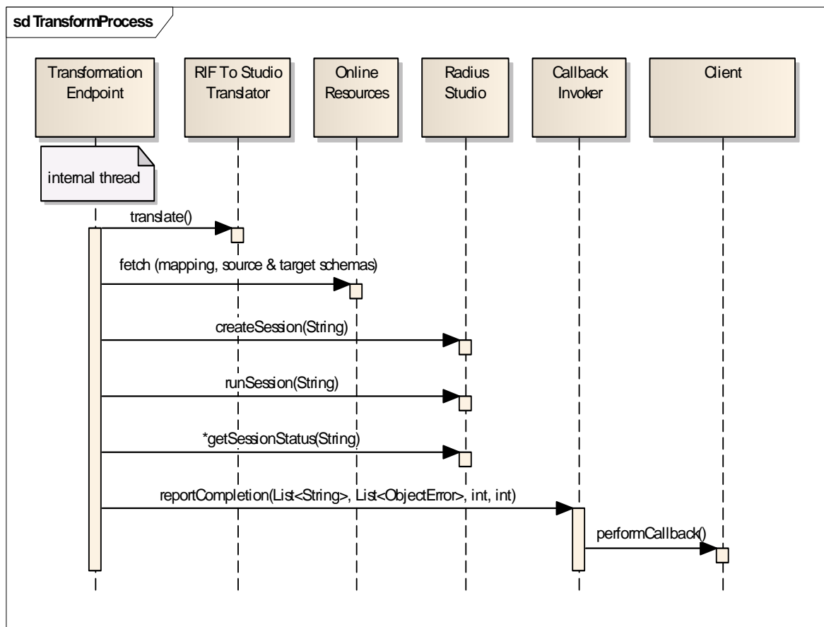
Figure 18 Transform process sequence diagram
