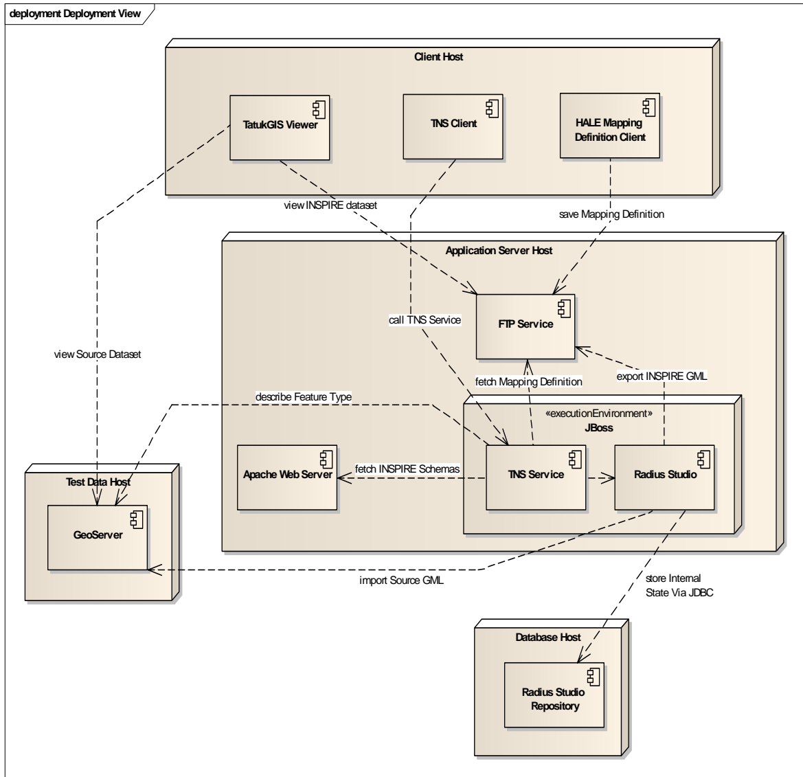
Figure 20 Prototype deployment view
