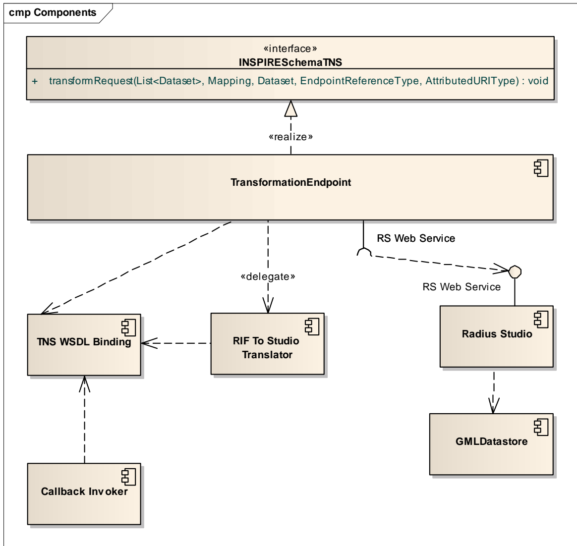
Figure 9 Prototype Schema Transformation Network Service sub components
