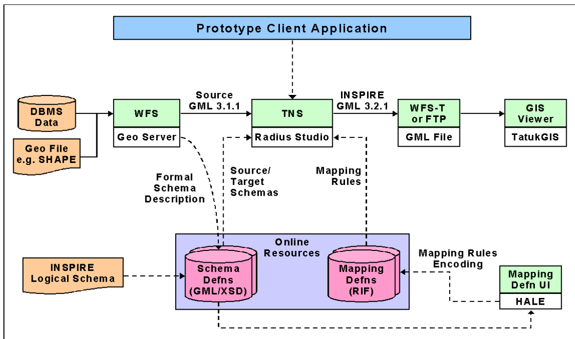
Figure 2 Prototype demonstrator components
