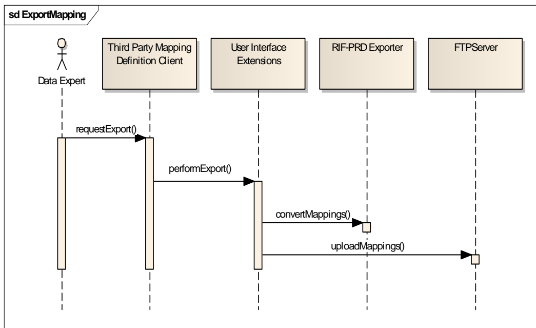
Figure 19 Export Mapping sequence diagram.
