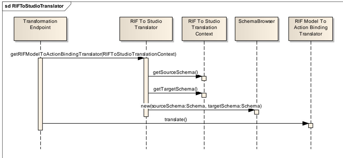
Figure 13 Process flow for the RIF To Studio Translator
