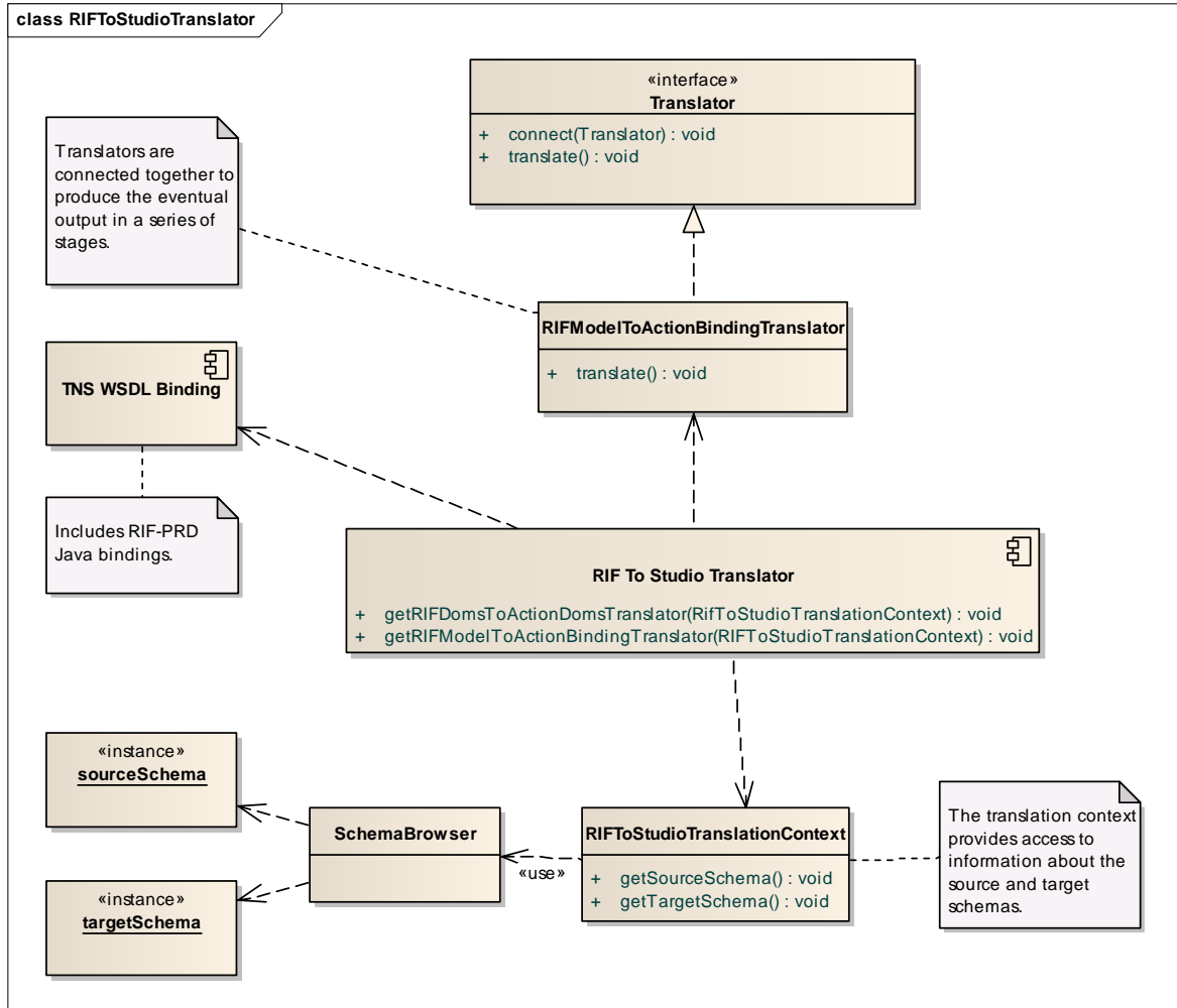
Figure 12 RIF To Studio Translator class diagram
