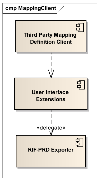
Figure 14 Prototype mapping client sub components
